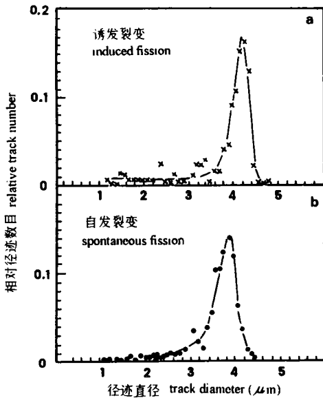
图 1 玻璃陨石中自发裂变与诱发裂变径迹直径的分布。自发裂变径迹最可几直径小于诱发裂变径迹最可几直径，表明自发裂变径迹曾因受热而衰退 Distributions of track diameters of induced fission(a) and spontaneous fission(b) in the tektite. The most probable value of diameter of spontaneous fission tracks is smaller than that of induced fission tracks, which shows that thermal fading of spontaneous fission tracks occurred in the tektite
