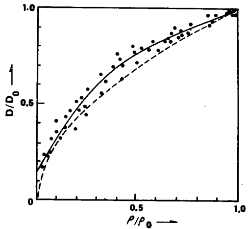
图 2 玻璃陨石中裂变径迹直径与径迹密度之间的对应关系 (Storzer et al. , 1969)。图中实线为通过实验点的光滑曲线，用这一曲线对玻璃陨石的年龄进行修正。虚线为用化学成分相同的人造玻璃的径迹蚀刻参数计算的曲线 Relationship between track diameter and track density in tektites (Storzer et al. , 1969). The solid curve is smoothed through the measured points. This curve was used to correct the tektite age. The dashed curve was calculated by using parameters measured on a synthetic tektite glass
