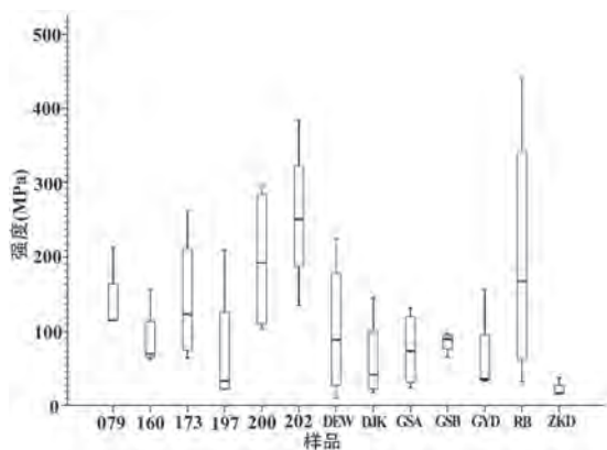
图6 不同产地石料的抗压强度 Fig.6 Raw material compressive strength from different sites
