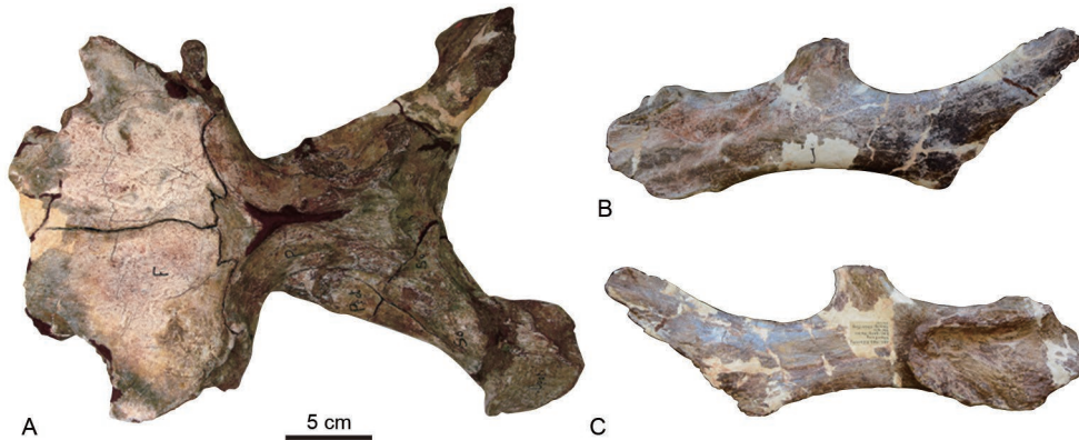
Fig. 4 Braincase and jugal of Tanius sinensis (PMU 24720) A. braincase in dorsal view; B–C. left jugal in lateral (B) and dorsal (C) views
