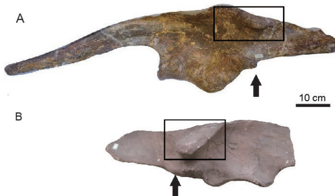
Fig. 5 Comparison between the ilia of Tanius sinensis and T. chingkankouensis in lateral view A. left ilium of T. sinensis (PMU 24720); B. right ilium of T. chingkankouensis (IVPP V 724)
